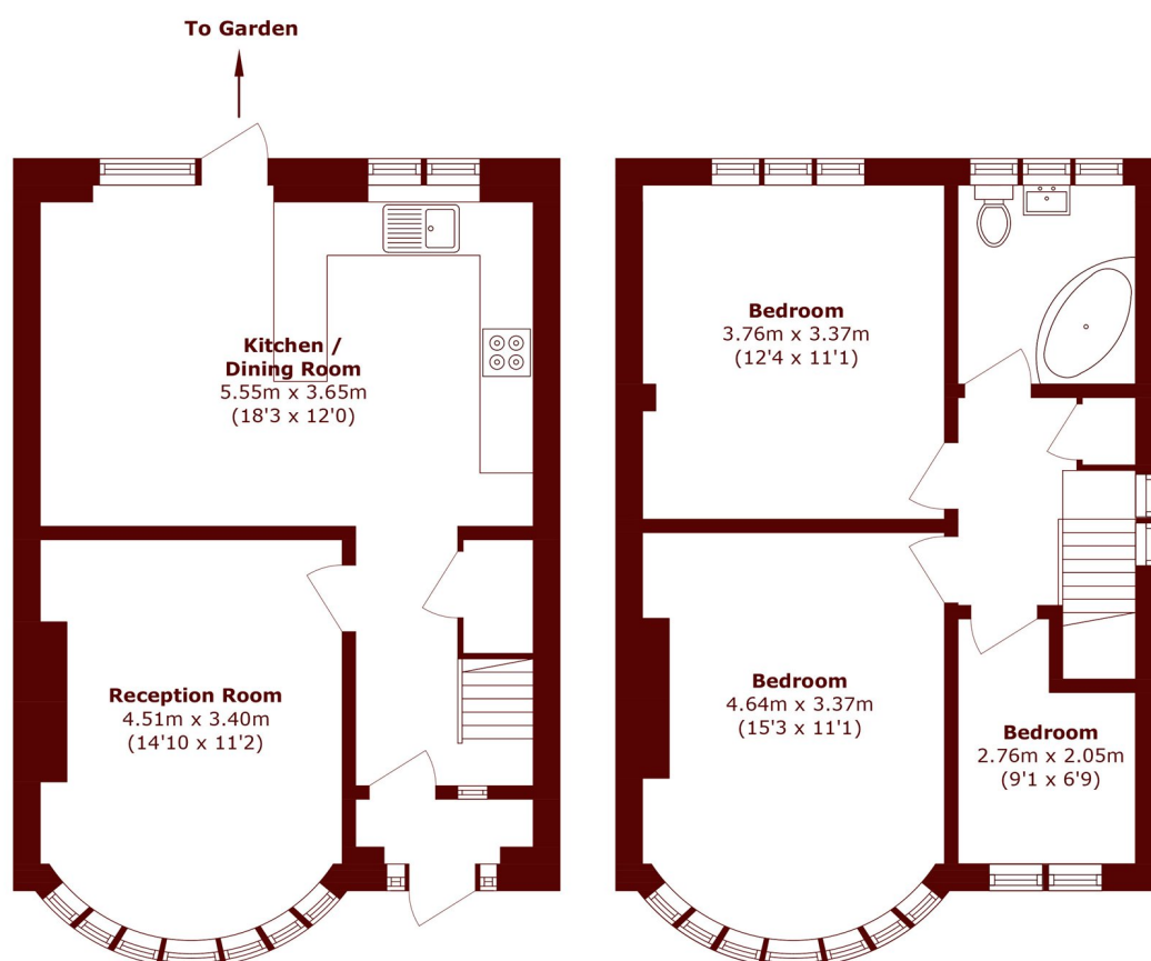
Ground Floor
