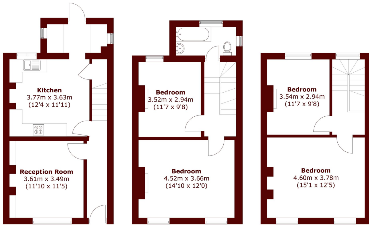
Ground Floor
