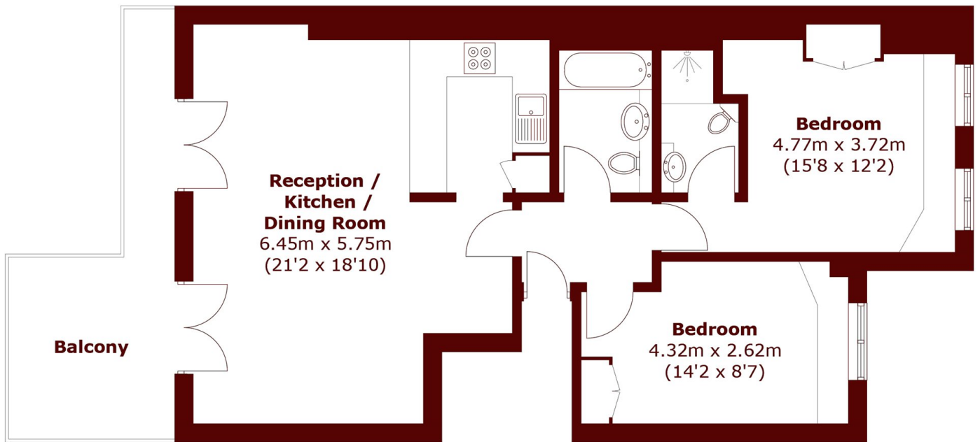
First Floor
